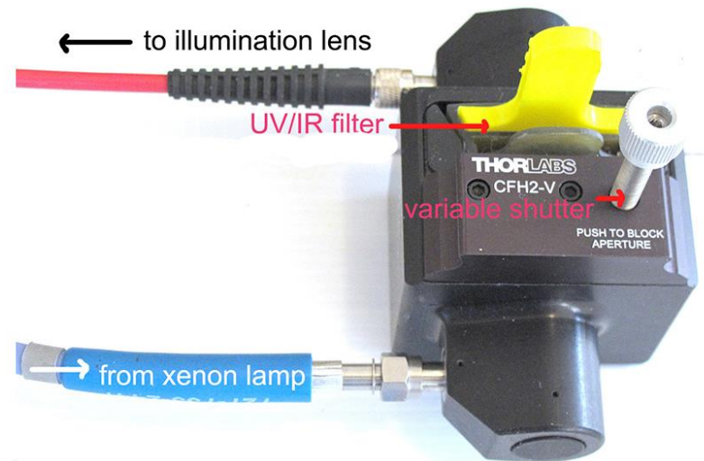
Thorlabs FOFMS Inline Filter Holder
